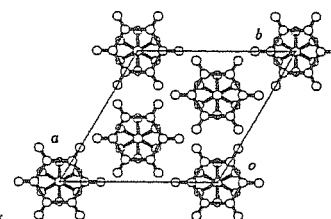
Fig. 2. Structure at 293K (Phase I)
