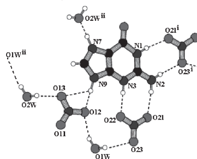
Fig.1 Intramolecular hydrogen bonding
