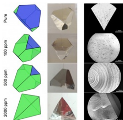
Figure 1. The evolution on changing crystal habit of NaBrO 3 crystals as a function of the S 2 O 6 2- concentration. The \{111\} - and \{-1-1-1\} -form faces, in blue and green respectively, swap importance in the final habit in function of the impurity level. Surface microtopography from the \{111\} -form faces show the roughness increase as the dopant level rises.
