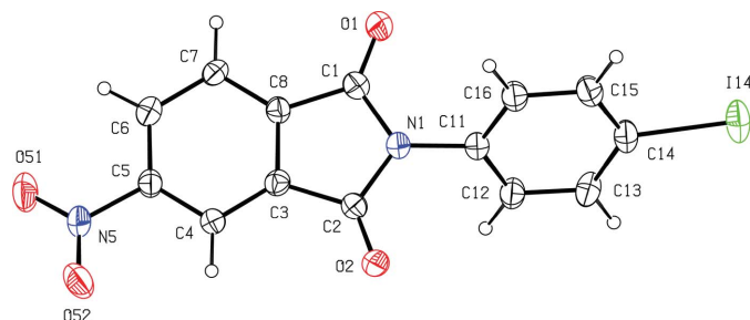
Figure 1 A molecule of (I) showing the atom-labelling scheme. Displacement ellipsoids are drawn at the 30% probability level.
