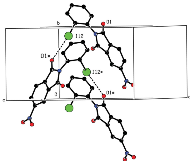
Figure 7 Part of the crystal structure of (III) showing the formation of an I \cdots O chain along [010]. For the sake of clarity, the H atoms have been omitted. The atoms marked with an asterisk (*) or a hash (#) are at the symmetry positions (\frac{1}{2} - x, -\frac{1}{2} + y, \frac{1}{2} - z) and (x, -1 + y, z) , respectively.
