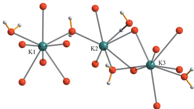
Figure 10 The coordination environments of the three independent potassium centres in the neutron-determined structure of (3).
