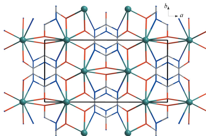
Figure 3 The crystal packing of (2), projected along the c axis.
