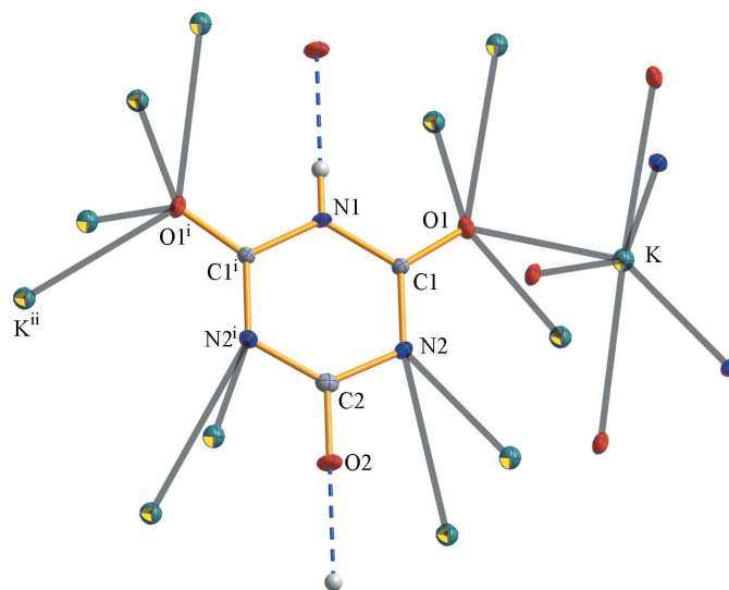
Figure 2 The structure of (2). Displacement ellipsoids are drawn at the 50% probability level, and the unique hydrogen bond is marked by a dashed line. [Symmetry codes: (i) -x, y, -z + \frac{1}{2} ; (ii) -x, -y + 1, z - \frac{1}{2} .
