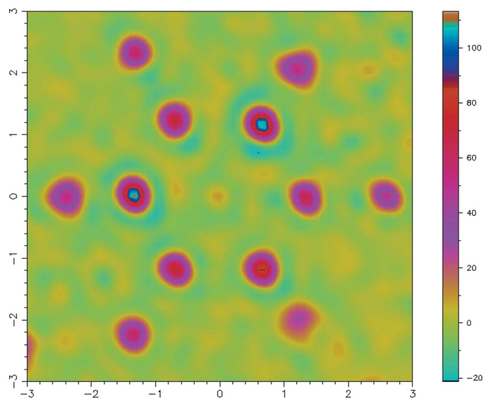
Figure 7 An F_{\text{obs}} Fourier map of the CYD_3 ligand as determined by neutron diffraction with the second model. The locations of all 12 atoms in the molecule are clear.
