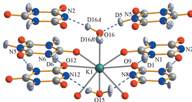
Figure 8 Part of the correct structure of (3) determined by neutron diffraction. The pseudo-mirror symmetry of the structure is approximately observed by all atoms except D5 and D16B. Their positions break the symmetry and result in extra weak reflections in the diffraction pattern which were not identified by X-ray diffraction.
