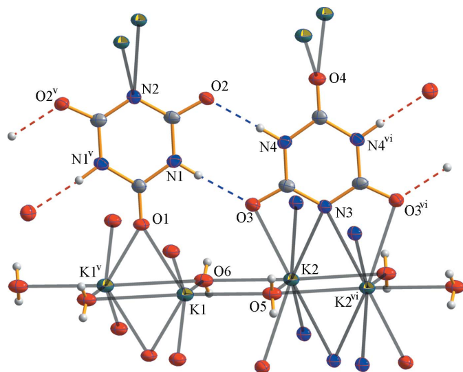
Figure 1 A partial packing diagram of (1). Displacement ellipsoids are drawn at the 50% probability level, and dashed lines indicate hydrogen bonding [symmetry codes (twofold rotation): (v) -x, y, -z ; (vi) -x + 1, y, -z + 1 ]. In all graphical representations of structures in the on-line version of the journal, bonds within ligands are orange, and bonds to metals are semi-transparent grey.
