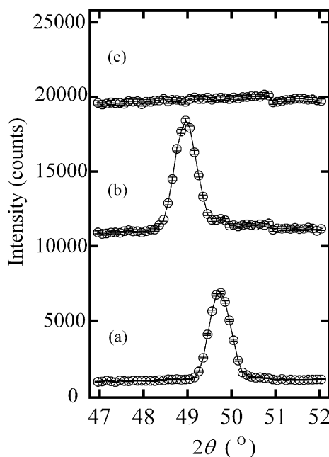
Figure 4 Neutron diffraction profiles around the 102_t reflection of \text{CeZrO}_4 solid solution measured at (a) 296, (b) 1542 and (c) 1831 K.
