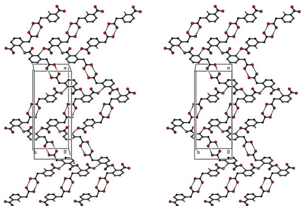
Figure 4 A stereoview of part of the crystal structure of (II), showing the formation of a sheet of R_2^2(8) and R_6^6(40) rings parallel to (10\bar{1}) . For the sake of clarity, H atoms not involved in the motifs shown have been omitted.
