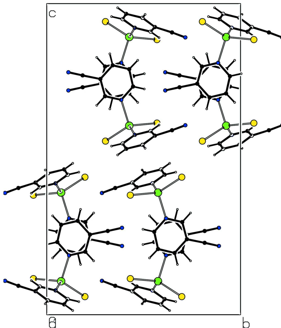
Figure 2 Packing diagram of the title compound with view along the a -axis.
