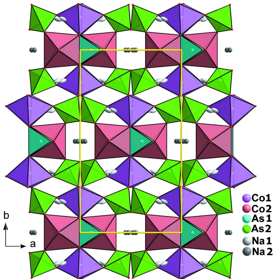
Figure 2 Polyhedron framework structure of (I) viewed along the c axis.
