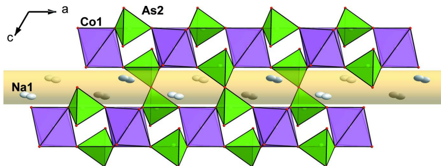
Figure 3 The polyhedral layers in the framework of (I); Na1 cations are on the periphery of tunnels parallel to [100] .
