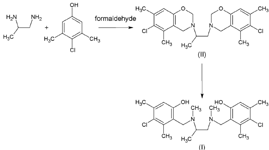
Figure 1 Synthetic route for the title compound.
