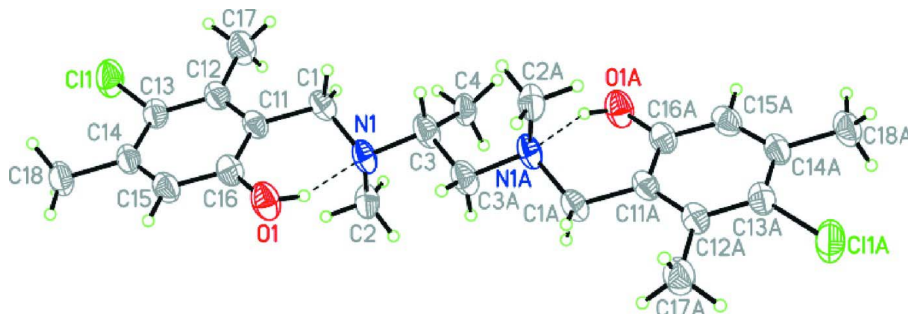
Figure 2 A perspective view of the title compound, showing the atom-numbering scheme. Displacement ellipsoids are drawn at the 50% probability level and H atoms are shown as small spheres of arbitrary radii. Only one of the two positions of the disordered methyl group is shown. Hydrogen bonds are drawn as dashed lines.
