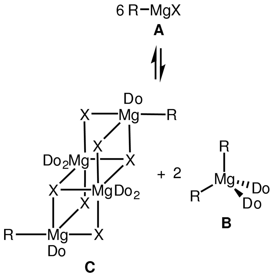
Figure 2 Grignard Compounds ( \text{RMgX} ) in Donor Solvents.
