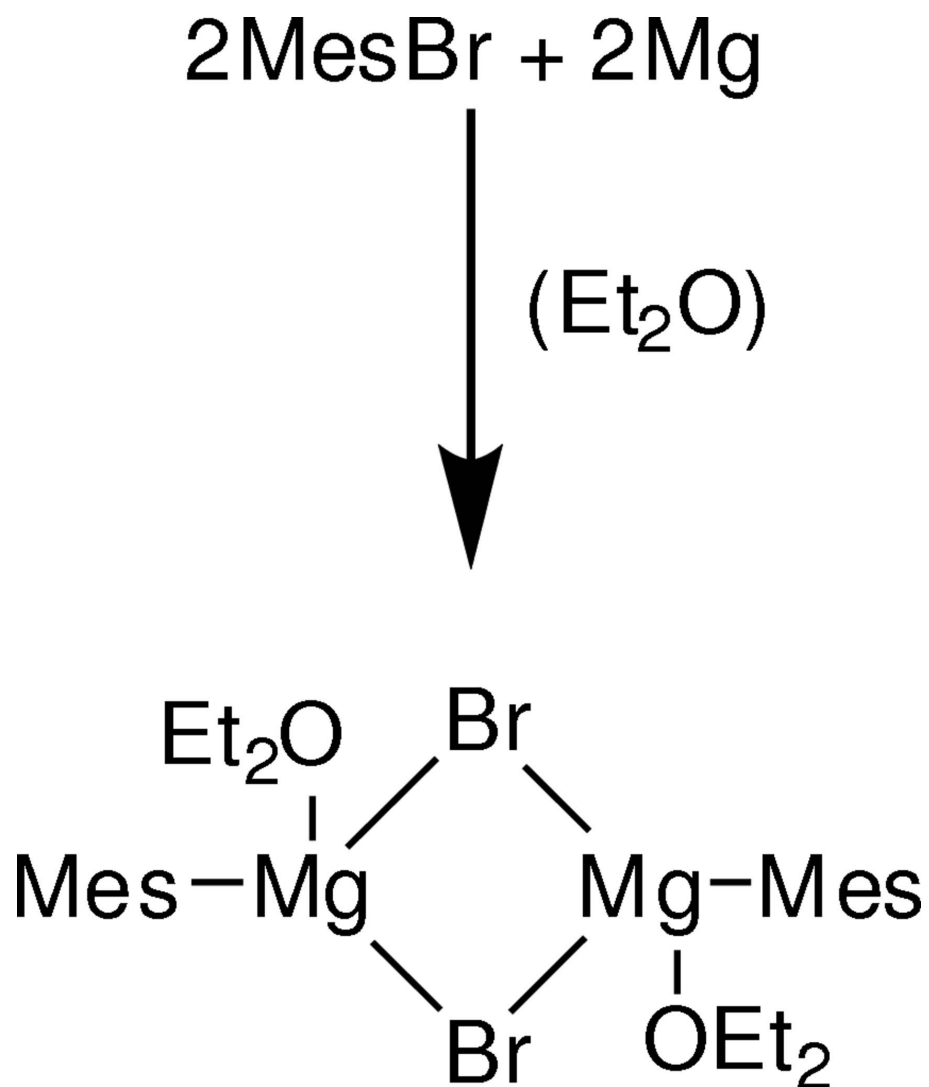
Figure 3 Synthesis of [\text{MgBrMes}(\text{OEt}_2)]_2 .
