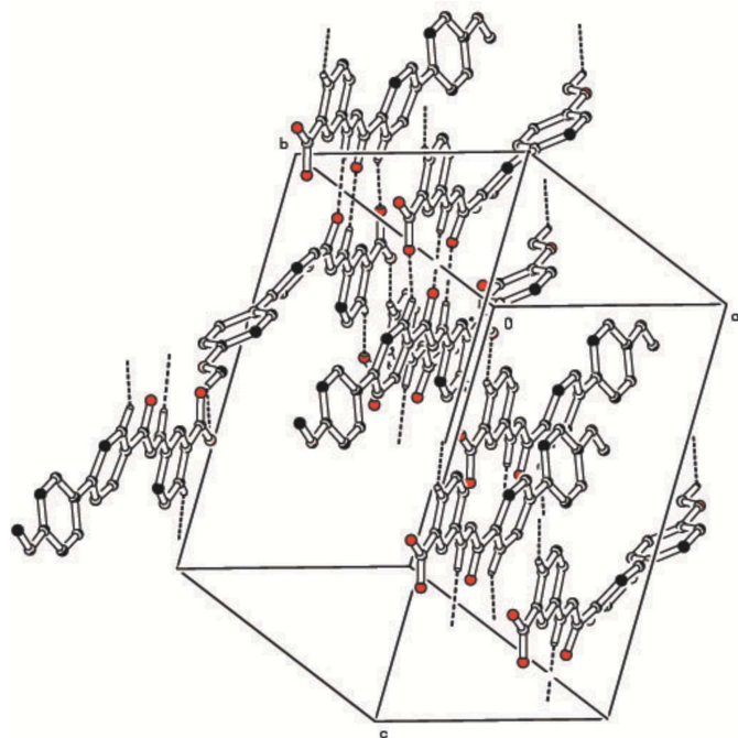
Figure 2 A partial view along the a axis of the crystal packing of the title compound, showing the C–H···O hydrogen bonds (dashed lines; see Table 1 for details; H atoms not involved in hydrogen bonding have been omitted for clarity).
