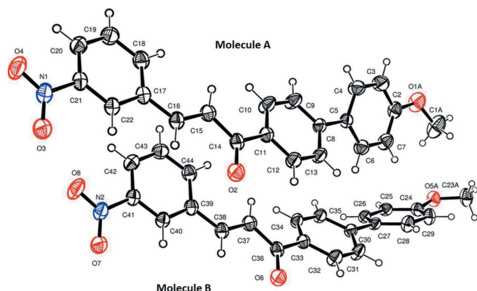
Figure 1 The molecular structure of the two independent molecules ( A and B ) of the title compound, with atom labelling. Displacement ellipsoids are drawn at the 30% probability level (the minor components of the disordered methoxy groups are not shown).
