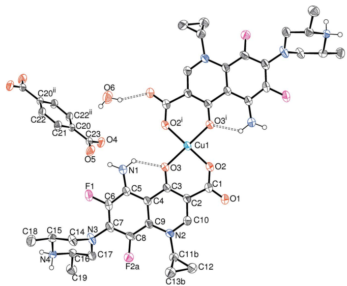
Figure 3 The molecular structure of (II) showing 50% probability displacement ellipsoids. Only one orientation of the disordered cyclopropyl ring is shown. Hydrogen bonds are shown as double-dashed lines. [Symmetry codes: (i) 1 - x, -y, 1 - z ; (ii) -x, -y, -z .]
