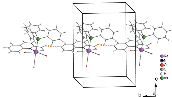
Figure 3 Chains of complexes, formed through \text{C7-H7}\cdots\text{O2} hydrogen bonds (dashed orange lines), parallel to the b axis.
