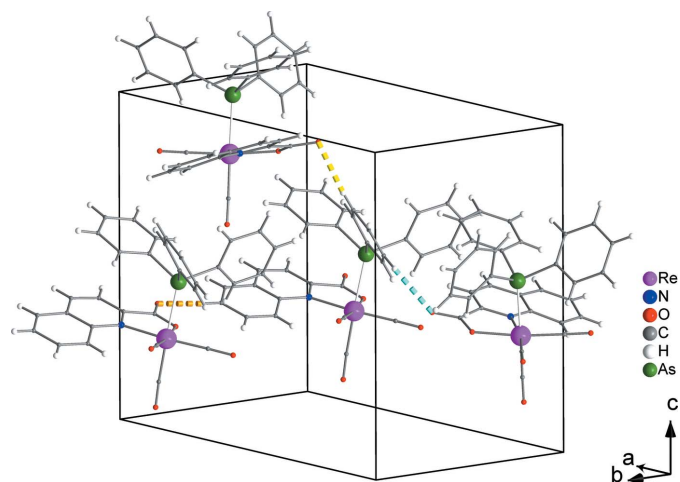
Figure 2 Weak intermolecular hydrogen bonds ( \text{C7-H7}\cdots\text{O2} , \text{C19-H19}\cdots\text{O2} and \text{C21-H21}\cdots\text{O2} ) between neighbouring complexes indicated by dashed orange, yellow and turquoise lines, respectively. Intramolecular hydrogen bonds are not shown for clarity.
