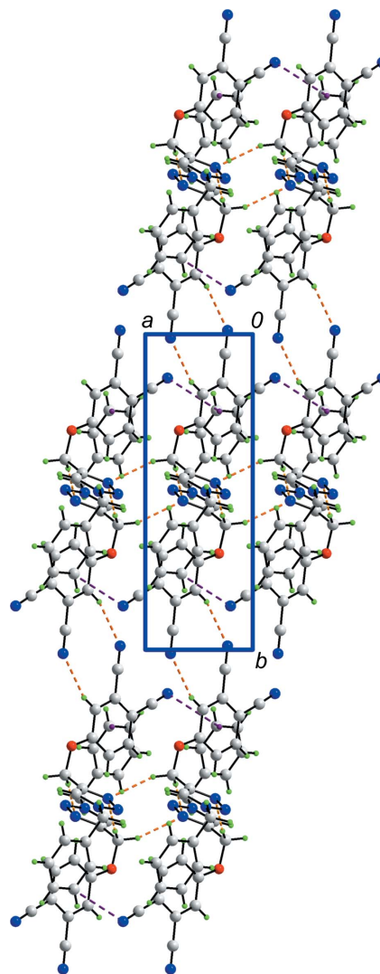
Figure 2 A view of the supramolecular layer in the ab plane in (I). The layer is sustained by C–H···N and C–H···N interactions shown as orange and purple dashed lines, respectively.
