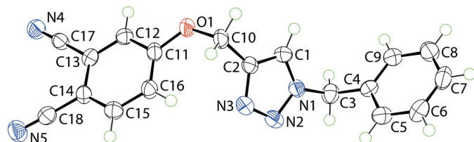
Figure 1 The molecular structure of (I), showing the atom-labelling scheme and displacement ellipsoids at the 70% probability level.
