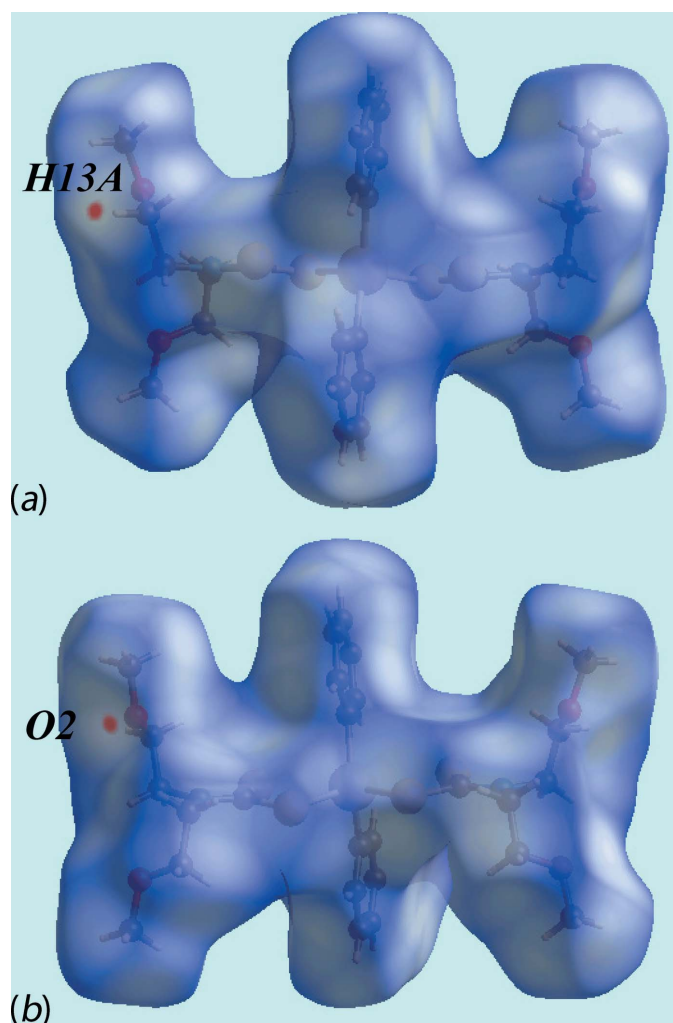
Figure 6 Views of Hirshfeld surfaces mapped over d_{\text{norm}} for (II).
