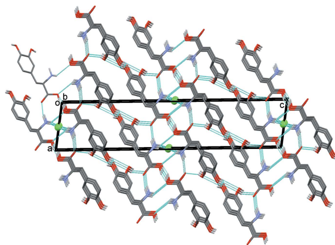
Figure 3 Crystal packing of the title molecular salt, (II), viewed along the b axis. The hydrogen bonds are shown as dashed lines (see Table 1), and C-bound H atoms have been omitted for clarity.
