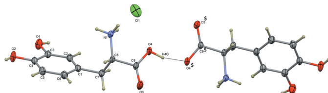
Figure 1 The molecular structure of the title molecular salt, (II), showing the atom labelling scheme [symmetry code: ($) -x + 3, y, -z + 1 ]. Displacement ellipsoids are drawn at the 50% probability level.
