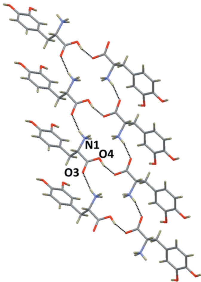
Figure 4 Part of the crystal structure of (II) showing the R_4^1(18) motifs formed through N-H\cdots O and O-H\cdots O hydrogen bonds (see Table 1).
