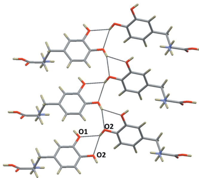
Figure 6 Adjacent dopa layers are interlinked by side chain–side chain interactions in (II) through intermolecular O-H\cdots O hydrogen bonds (see Table 1).
