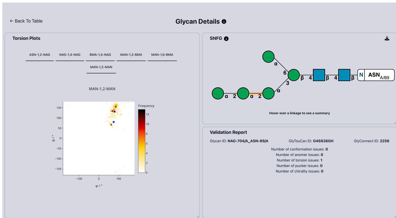
Figure 4 Right: detailed information about the glycan attached to Asn89 in PDB entry 3qyp (Kommoju et al. , 2011) after remodelling and refinement. Two additional \alpha -mannose sugars were added to the chain and the conformational issues of the deposited \alpha 1,2-mannose were corrected. Left: linkage torsion angles panel, which highlights the current torsion angles for this linkage (blue crosses) in relation to the previously reported torsional landscape.
