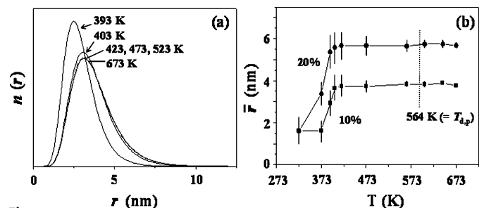
Figure 4 (a) Porogen and pore radii and their radius distributions determined from the GISAXS analysis of the in-plane scattering profile data in Figs. 3(a) and 3(b). (b) Average radii of porogens and pores in the PMSSQ films determined from the GISAXS analysis of the in-plane scattering profile data obtained for the films loaded with 10 and 20 wt% PCL6 porogen.
