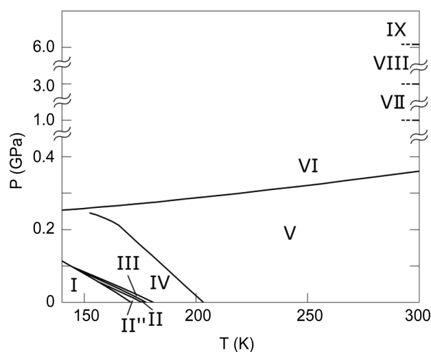
Figure 2 The phase diagram of thiourea. Phase transitions were first reported by Bridgman (1938) (V → VI), Goldsmith & White (1959) (I → II, II → III, III → IV and IV → V), Moudden et al. (1979) (phase II'') and Banerji & Deb (2007) (VI → VII, VII → VIII and VIII → IX). Phase boundaries were investigated by Klimowski et al. (1976) and Benoit et al. (1983). Phase V crystallizes in Pnma (Wyckoff & Corey, 1932) and phase I in Pmc 2 (Goldsmith & White, 1959).
