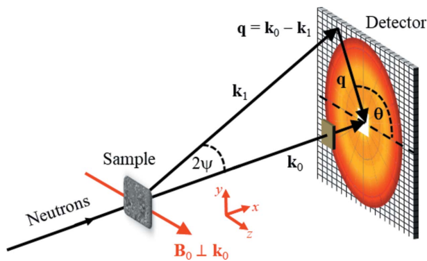
Figure 2 A sketch of the neutron scattering geometry. The applied magnetic field \mathbf{B}_0 \parallel \mathbf{e}_z is perpendicular to the wavevector \mathbf{k}_0 \parallel \mathbf{e}_x of the incident neutron beam ( \mathbf{B}_0 \perp \mathbf{k}_0 ). The momentum transfer or scattering vector \mathbf{q} is defined as the difference between \mathbf{k}_0 and \mathbf{k}_1 , i.e. \mathbf{q} = \mathbf{k}_0 - \mathbf{k}_1 . SANS is usually implemented as elastic scattering ( k_0 = k_1 = 2\pi/\lambda ) and the component of \mathbf{q} along the incident neutron beam, here q_x , is much smaller than the other two components, so that \mathbf{q} \cong [0, q_y, q_z] = q[0, \sin\theta, \cos\theta] . This demonstrates that SANS predominantly probes correlations in the plane perpendicular to the incident beam. For elastic scattering, the magnitude of \mathbf{q} is given by q = (4\pi/\lambda) \sin(\psi) , where \lambda denotes the mean wavelength of the neutrons and 2\psi is the scattering angle. The angle \theta = \angle(\mathbf{q}, \mathbf{B}_0) is used to describe the angular anisotropy of the recorded scattering pattern on the two-dimensional position-sensitive detector.
