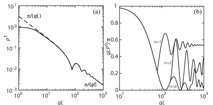
Figure 2 (a) The form factor of a single helix according to the exact (solid curve) and limiting (dashed curve) formulas. (b) The normalized form factor qLP^n/\pi pertaining to single ( n = 1 ), diametrically symmetric ( n = 2 ) and sixth-order ( n = 6 ) helices. Notice that qLP^n/\pi tends to L/(nl) for qL \rightarrow \infty . For both (a) and (b), the parameters are radius r = 5 , pitch 2\pi p = 20 and helix length L = 250 .
