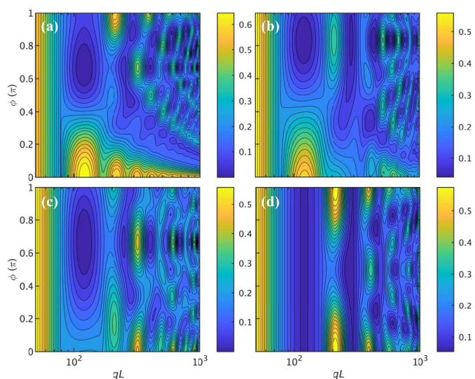
Figure 5 (a) A contour plot of the normalized form factor qLP^3/\pi pertaining to a triple helix with variable enclosed angle \phi_1 = \phi_2 = \phi . (b)–(d) As in (a) but for the general case with variable angle \phi_1 and fixed angles \phi_2 = \pi/3, 2\pi/3 and \pi , respectively. For all plots, the parameters are radius r = 5 , pitch 2\pi p = 20 and helix length L = 250 .
