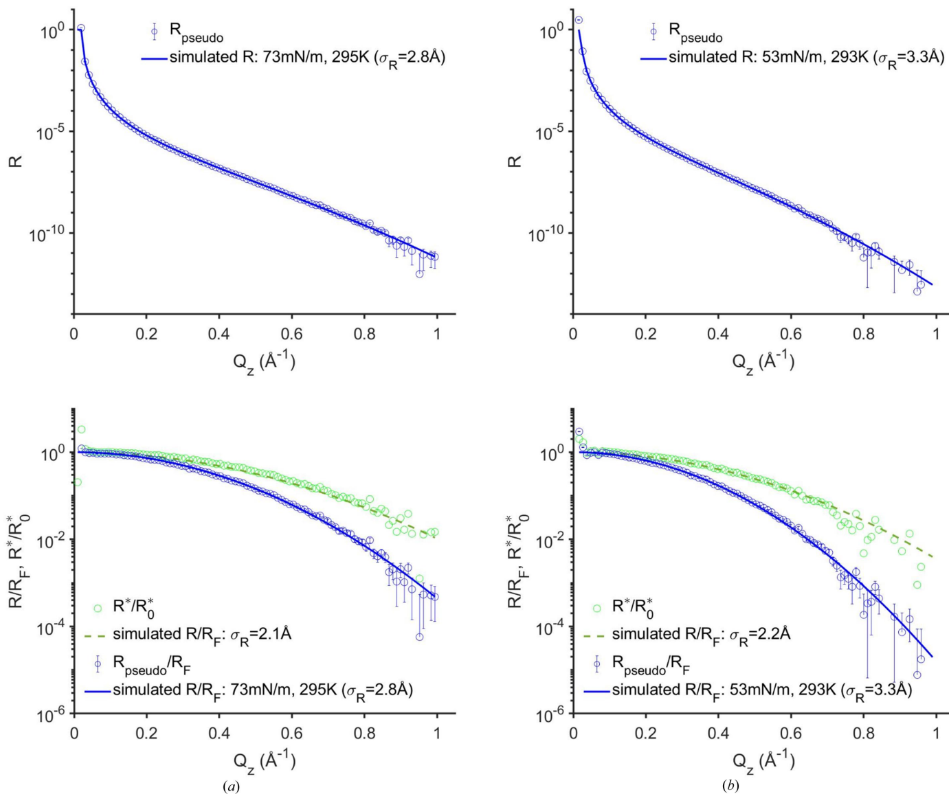
Figure 4 The diffuse scattering data measured by GIXOS at Q_{xy}|_{\beta=0} = 0.03 \text{ \AA}^{-1} (see Fig. 2 caption) and the pseudo-reflectivity data derived from it, from the water surface (a) and from the surface of the mixture of water with 10 vol% ethanol (b). The blue circles (with error bars) show R_{\text{pseudo}} = R^*/r (top) and R_{\text{pseudo}}/R_F (bottom) along with the simulated R/R_F predicted by the CWM (solid blue lines, see text). The green circles correspond to the normalized diffuse scattering, R^*/R_0^* , where R_0^* = \frac{1}{4} [t(\alpha)]^2 \rho_{b,\infty}^2 k_B T \Delta \beta \Delta 2\theta / [\sin(\alpha) \gamma Q_{xy}^2] is the Q_z -independent pre-factor of R^* [equation (6)]. The normalized diffuse scattering follows R/R_F with a smaller r.m.s. roughness predicted by the CWM (green dashed line, see text).
