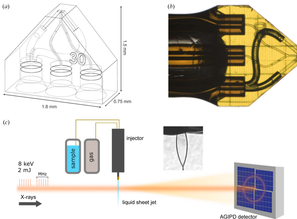
Figure 1 (a) CAD-drawing of 3D-printed sheet jet nozzle design. Two liquid inlets converge to form a single channel ( 30 \times 30 \mu\text{m} ) above the nozzle tip. Gas channels ( 50 \times 50 \mu\text{m} ) are split from a single inlet and opposed at an 80^\circ angle. (b) Image of assembled sheet jet nozzle. (c) Experimental setup at the EuXFEL SPB/SFX nanofocus beamline.
