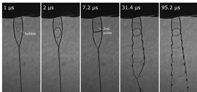
Figure 3 Stroboscopic visualization of sheet jet explosion on exposure to the nanofocus XFEL beam (141 kHz) at various time delays following the initial X-ray pulse as captured by the side view microscope camera within the experimental chamber. The fluid velocity within the liquid sheet was estimated by following the movement of the bubble over time. Note that the flat section of the jet is oriented at 45° with respect to the camera.
