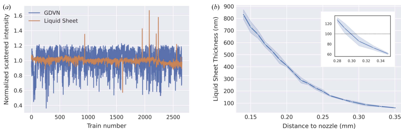
Figure 2 (a) The integrated AGIPD detector response normalized by incoming X-ray intensity for all trains (176 pulses) over a representative 5 min measurement window for the liquid sheet jet and GDVN. (b) Thickness dependence of the primary sheet section while scanning vertically away from the nozzle tip towards the lower rim. The shaded region reflects a measurement error of one standard deviation. A magnified view of the thinnest region is shown in the inset.
