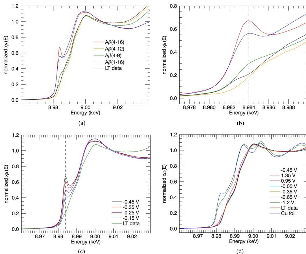
Figure 6 (a) Room-temperature XANES-EC spectra for Cu:Abeta at a reduction potential of -0.45 V. Reducing potentials for Cu II :Abeta 1-y peptide complexes in the literature are in the range of 0.28 – 0.34 V (Guilloureau et al. , 2007; Jiang et al. , 2007). Changes in the potentials depend upon the time allowed for the equilibrium of species. (b) Enlarged XANES spectra showing the Cu I characteristic peak at 8984 eV corresponding to the 1s – 4p transition. (c) Room-temperature XANES-EC spectra for Cu:Abeta 4-16 at a series of reducing potentials from -0.15 to -0.45 V. (d) Room-temperature XANES-EC spectra for Cu:Abeta 4-12 at different reducing potentials from -0.05 to -1.20 V. Plots are compared with the low-temperature (LT) and Cu-foil XANES spectra.
