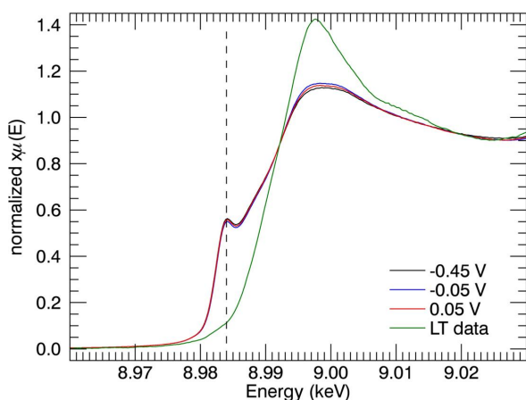
Figure 7 Room-temperature XANES-EC spectra for Cu:Abeta 1-16 at reducing potentials from 0.05 to -0.45 V. The Cu I characteristic peak is observed at 8984 eV corresponding to the 1s – 4p transition. The pre-edge peak heights are slightly smaller than the reported spectra for reductions by ascorbate (Streltsov et al. , 2008).
