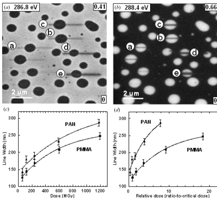
Figure 4 Evaluation of radical migration in a PMMA-blend-PAN microphase-separated film. (a) Optical image at 286.8 eV (PAN is white). (b) Optical density image of the same region at 288.4 eV (PMMA is white). The lines labeled a , b , c , d , e were exposed to various doses at 320 eV prior to recording these images. (c) Plot of the average width of the damage lines in the PAN and PMMA material as a function of the dose. The data points are the measured line width (FWHM) at the indicated radiation doses for PMMA and PAN, respectively. The lines are fits of those data points to w = w_0 + a \exp(d/d_c) . (d) Plot of the average width of the damage lines in the PAN and PMMA material as a function of ratio-to-critical dose ( 60 \times 10^6 Gy for PMMA, 150 \times 10^6 Gy for PAN).
