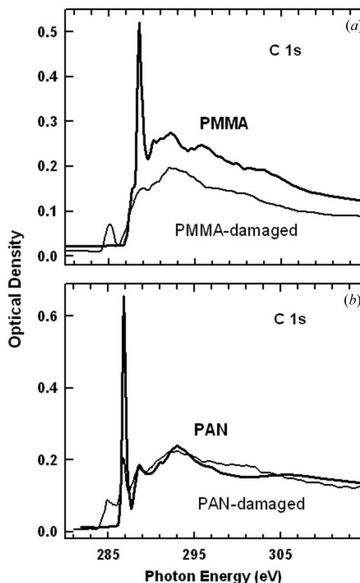
Figure 1 C 1s near-edge X-ray absorption fine structure (NEXAFS) spectra of undamaged and damaged PMMA (a) and PAN (b).
