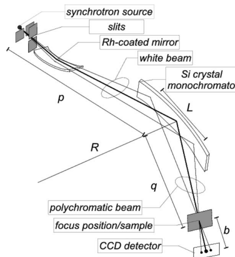
Figure 1 Schematic view of the EDXAS set-up showing the synchrotron source, the vertically focusing mirror, the bent crystal monochromator and the detector. The photon energy-direction correlation is transformed into an energy-position correlation along the horizontal axis of the detector.
