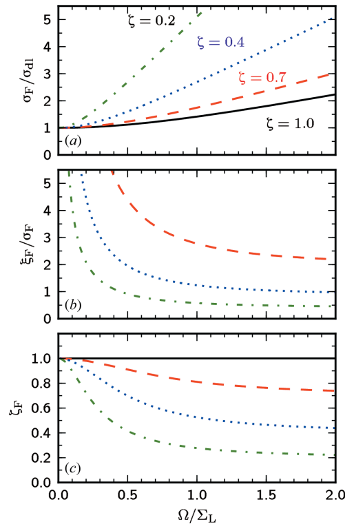
Figure 5 The normalized focus size \sigma_F/\sigma_{dl} (a), transverse coherence length \xi_F/\sigma_F (b), and global degree of coherence \zeta_F in the focus (c) as functions of the ratio \Omega/\Sigma_L . Different values of the global degree of coherence at the source \zeta = 1.0, 0.7, 0.4 and 0.2 are considered.
