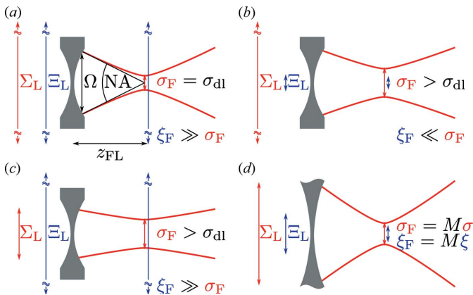
Figure 4 (a) Focus is diffraction-limited \sigma_F = \sigma_{dl} if the beam size \Sigma_L and transverse coherence length \Xi_L are larger than the lens aperture \Omega . (b, c) Focus size is larger than the diffraction limit if the coherence length (b) or beam size (c) incident on the lens is smaller than the aperture. (d) For a very large aperture the focus is a demagnified image of the source.
