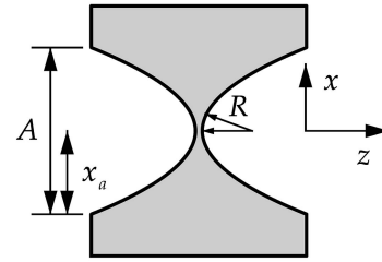
Figure 1 Parameters of the X-ray double concave lens and the coordinate axes.
