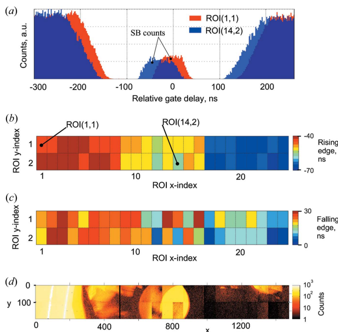
Figure 2 (a) Count-rate histograms as a function of gate delay for two different ROIs. (b) PILATUS 300K-W photosensor area divided on a grid of 24 \times 2 ROIs. The color code corresponds to the position of the single-bunch histogram left shoulder. (c) Same as in (b) but the color code corresponds to the position of the single-bunch histogram right shoulder. (d) Detector image of integrated photon counts after 10^7 gated exposures taken at zero relative gate delay. The data are taken from a real experiment.
