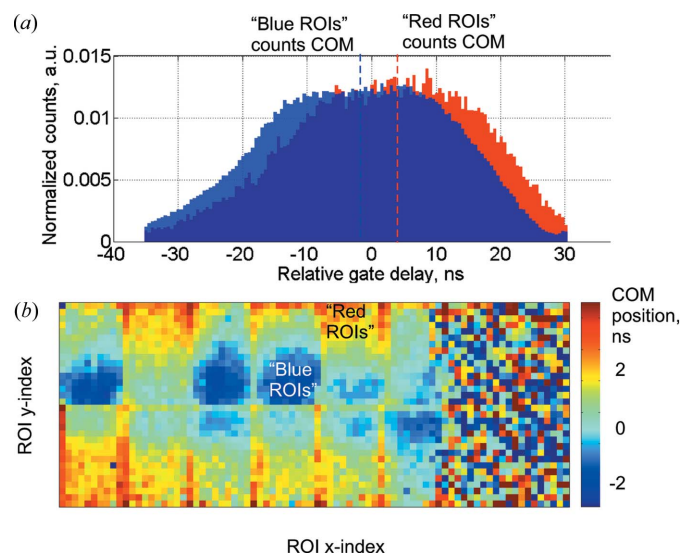
Figure 3 (a) Two overlaid count-rate histograms as a function of gate delay for the ‘blue’ and the ‘red’ ROIs as indicated in (b). Dashed vertical lines indicate the ‘center of mass’ (COM) position of the corresponding histogram. (b) PILATUS 100K photosensor area divided on a grid of 82 \times 32 ROIs. The color code corresponds to the COM position of the single-bunch histogram. The statistical noise seen on the right-hand side of the photosensor area is due to the much lower X-ray photon hit rate in this region.
