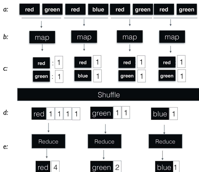
Figure 4 A simple word count example to explain processing under the MapReduce framework. (a) The input is a series of words in a single document. (b) Each map scans part of the input. (c) An intermediate count of words is emitted by each map as a key-value pair. The word itself is the key and the count of its occurrence is the value. (d) Shuffle combines the intermediate key-values and passes them to reduce, where each reduce function obtains a distinct key along with all the intermediate values associated with that key. (e) Reduce computes the final count.
