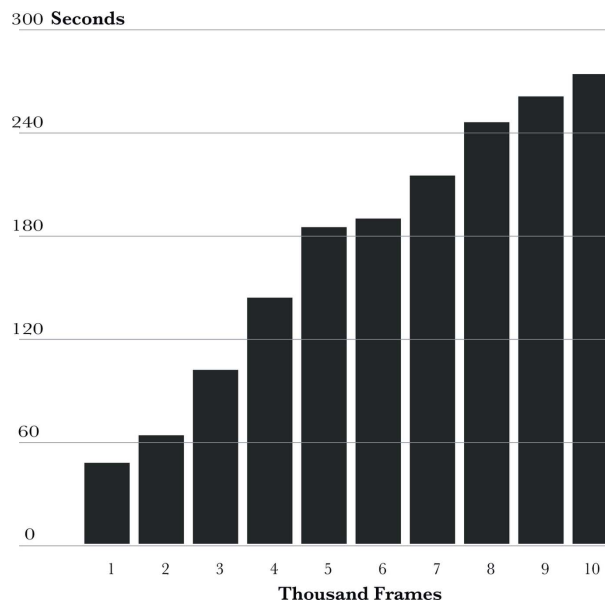
Figure 9 Time (in seconds) to compute the two-time correlation for a given data size.
