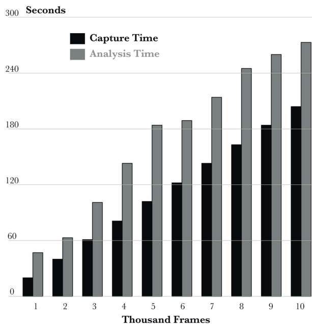
Figure 10 Time comparison (in seconds) against number of frames for recording and analyzing data using the two-time auto-correlation algorithm. The analysis and capture times are stacked in the same plot for better comparison.
