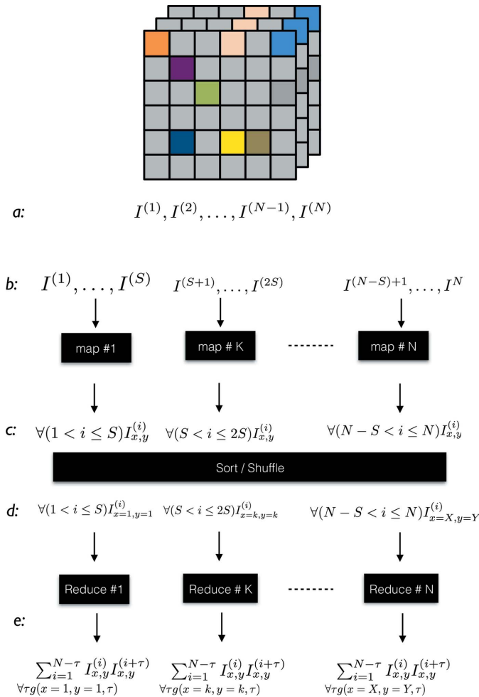
Figure 6 (a) The area detector writes images as a series of frames. (b) The data are stored in a distributed filesystem where the data are split into blocks of equal size, S . These blocks are processed by individual maps. Each map handles a unique split of the data. (c) The pixel-intensity data per frame is emitted as intermediate data. (d) The framework combines pixel intensities for all frames for a given pixel and passes it to a reducer. (e) The reduce processes compute the auto-correlation of pixel-intensities across time.
