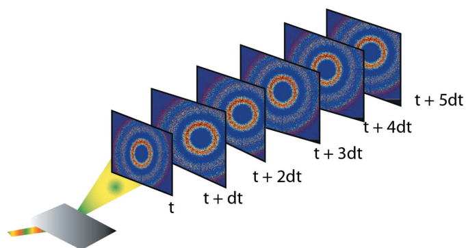
Figure 1 Conceptual representation of the time series nature of X-ray data captured by the area detector. Each frame consists of a fixed number of pixels and is separated by a fixed time. The correlation is computed for each pixel in the time domain and then averaged over a group of nominally equivalent pixels.
