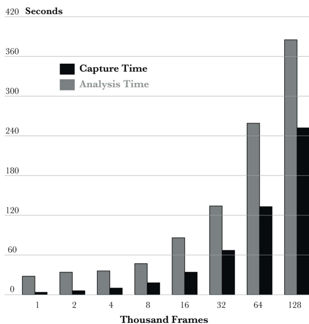
Figure 8 Time (in seconds) to compute the multi-tau auto-correlation for a given data size in comparison with the time taken for collecting the same dataset. The analysis and capture time are shown side-by-side for better comparison.
