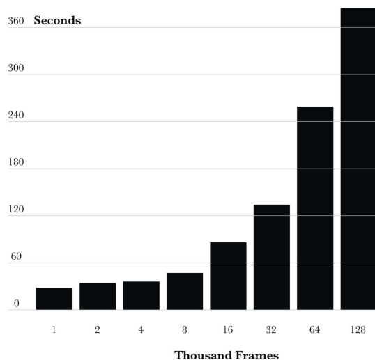
Figure 7 Time (in seconds) to compute multi-tau correlations for data sets of different sizes.
