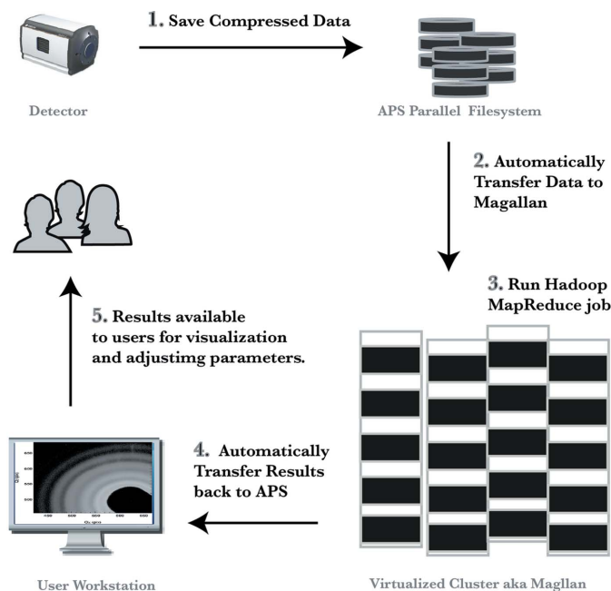
Figure 11 The virtualized XPCS acquisition and analysis workflow system in use at the APS. These components are loosely connected via a well defined HDF5 file interface and a message-based workflow pipeline. (1) The detector data acquisition system writes data directly to a parallel file system located at the APS. (2) The workflow pipeline automatically transfers data from the APS to the Magellan resource over 2 × 10 Gb s -1 network links. (3) The Hadoop MapReduce -based autocorrelation job and subsequent fitting routines are run on the Magellan resource. (4) Reduced data are automatically transferred back to the APS. (5) The user views output visualizations and may adjust experiment parameters for subsequent acquisitions.
