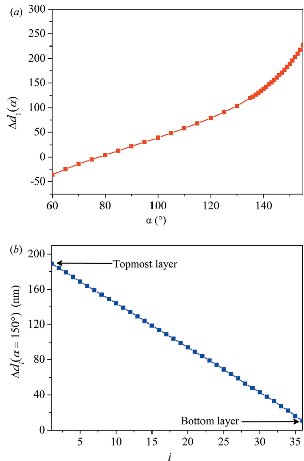
Figure 2 Dependences calculated for a W/B 4 C grating with \varphi = 1.76^\circ and \beta = 20^\circ : (a) shift of the grating topmost boundary profile versus the deposition flux incidence angle; (b) shift of the grating boundary profile ( \alpha = 150^\circ ) versus the number of layers.
