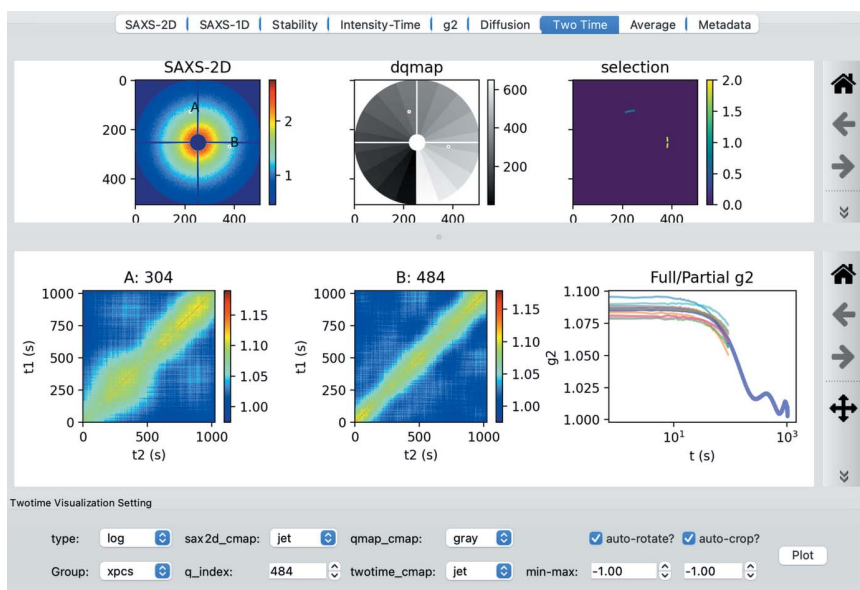
Figure 5 Two-time correlation visualization. The upper panels show the scattering pattern as well as the dynamical Q -map that allows users to select regions (A and B) of interest to explore. The lower panels show the two-time maps for the selected points. The full (blue) and partial (red) g_2 curves for selection B are also displayed.
