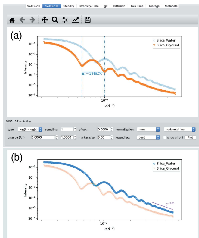
Figure 2 1-D small-angle scattering visualization. Users can draw horizontal lines (vertical dashed lines help users locate peaks/valleys) to estimate the structure size as shown in (a) or draw slopes to estimate the power-law decay constant as shown in (b).
