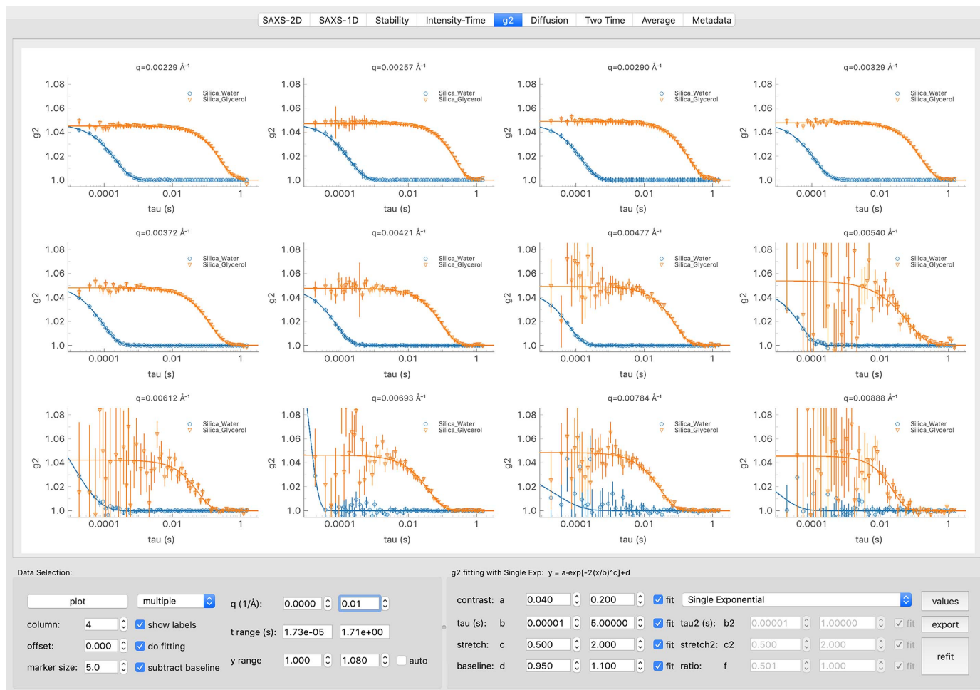
Figure 4 Multi-tau visualization and modeling. Users can customize the plot ranges, offset and the layout. Two widely used fitting models are included. Additional details about this module can be found in the text.
