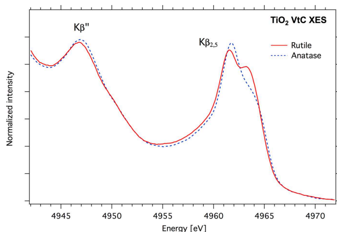
Figure 11 XES VtC spectrum of \text{TiO}_2 in the form of rutile and anatase.
