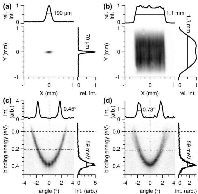
Figure 8 Small spot (a, c) versus large spot (b, d) setting of the refocusing mirror. (a, b) Distribution of X-ray flux on a scintillator plate at normal incidence at the designated sample position. (c, d) ARPES measurements of the Shockley state of the Cu(111) surface at h\nu = 70 eV. The measurements were taken in fixed-energy mode at a pass energy of 10 eV and integrated over 10 min. The line graphs show the integrals over one dimension (a, b), or the profiles along the dash-dotted lines (c, d), respectively. Full width at half-maximum is indicated.
