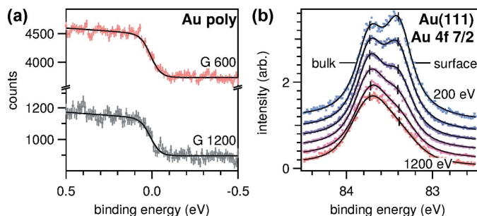
Figure 7 (a) High-resolution XPS spectra at the Fermi edge of polycrystalline gold measured at h\nu = 400 eV. Dots are electron counts integrated over the 60^\circ acceptance angle of the analyser with error bars estimated according to the Poisson distribution. Lines are curve fits of a Fermi function assuming, to first order, a linear increase of the density of states below E_F . (b) High-resolution XPS spectra of the Au 4f_{7/2} peak of a single-crystal Au(111) surface measured at a series of photon energies between 200 and 1200 eV. Solid lines are curve fits of two Voigt profiles. The weighted mean of the binding energy of the bulk peak is E_B = (83.73 \pm 0.01) eV, and the surface core-level shift is (0.329 \pm 0.001) eV. The spectra are normalized to the area of the bulk peak and vertically offset for clarity.
