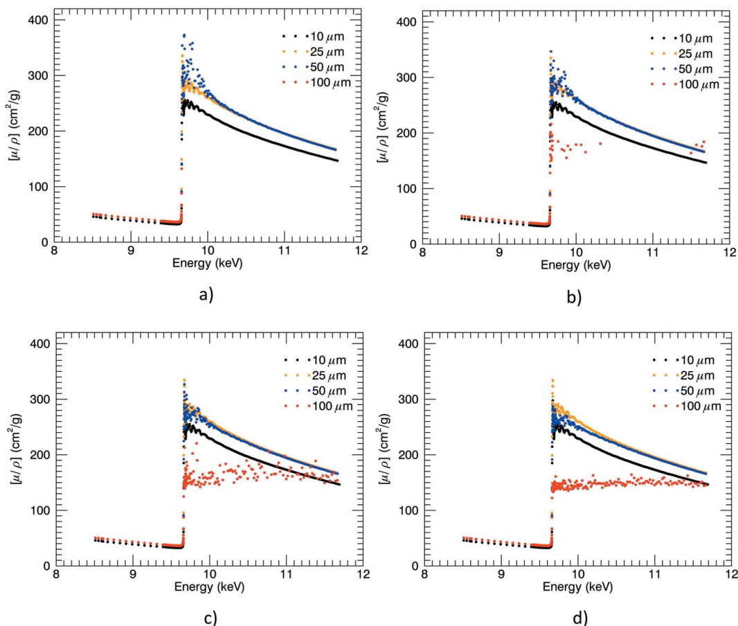
Figure 7 The mass attenuation coefficient of zinc from foils of different thickness: (a) without dark current offset ( i.e. assuming the determinations of dark current are correct to within 0.5 counts); with dark current offset of (b) 1 counts s -1 , (c) 4 counts s -1 and (d) 6 counts s -1 . The oscillatory pattern above the edge was not observable for the thickest foil, confirming that the measured dark currents were accurate to within 0.5 counts.
