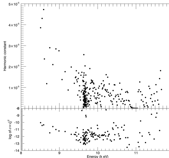
Figure 14 The effective harmonic for the X-ray beam across all energies in the experiment. The value is always less than 5 \times 10^{-5} and lies between zero and 1 \times 10^{-5} for most of the energies above the edge energy.
