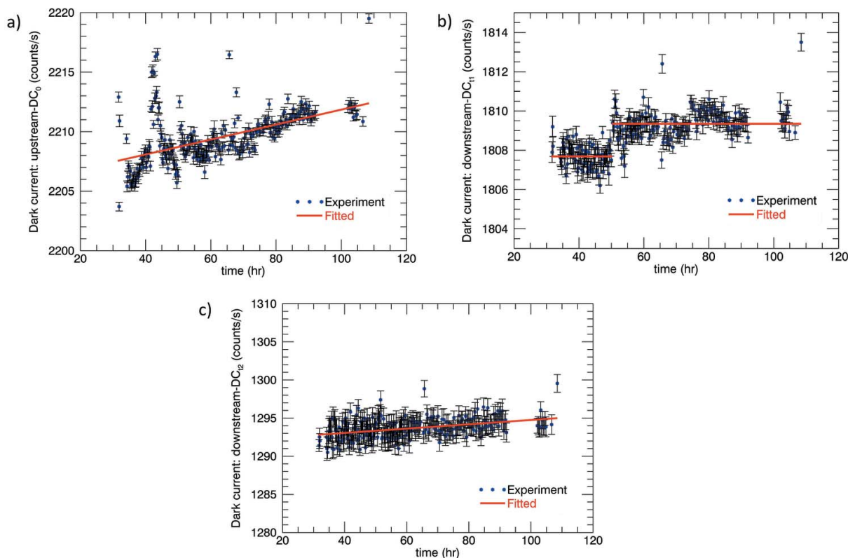
Figure 4 Dark current (DC) of (a) the upstream, (b) the first downstream and (c) the second downstream ion chamber versus time with uncertainties obtained from ten repetitions of measurements. A slightly increasing linear function has been fitted to the experimental measurements of the upstream ion chamber with \chi_r^2 of 3. DC measurements of the first downstream ion chamber were linearly fitted with \chi_r^2 of 1 across two ranges of time. DC of the second downstream ion chamber were fitted with a \chi_r^2 of 1.4. Fitted data are plotted in red.
