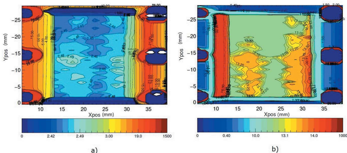
Figure 8 Attenuation maps of the 50 \mu\text{m} foil at (a) 8.61 keV and (b) 12.9972 keV. The low-energy map highlights the edges of the plastic holder while the higher-energy map highlights the edges of the sample foil. Circular spots indicate locations of the screws used to mount the foil. The vertical axis is Y_{\text{pos}} .
