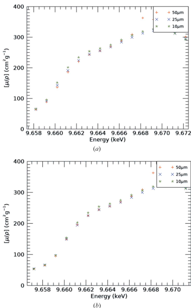
Figure 17 Plots showing the absorption edge (a) before and (b) after the correction for the effect of bandwidth. While the 10 \mu\text{m} data do not align perfectly with the 25 and 50 \mu\text{m} samples, there is still a significant improvement in the agreement between the different foils.
