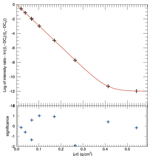
Figure 13 Harmonic contribution to the attenuation of aluminium foils at the daisy wheels for 9.7596 keV. The model equation provides a harmonic constant of 1.85 \times 10^{-5} by fitting experimental data with a \chi_r^2 of 1.66, i.e. almost at the limit of measurement.
